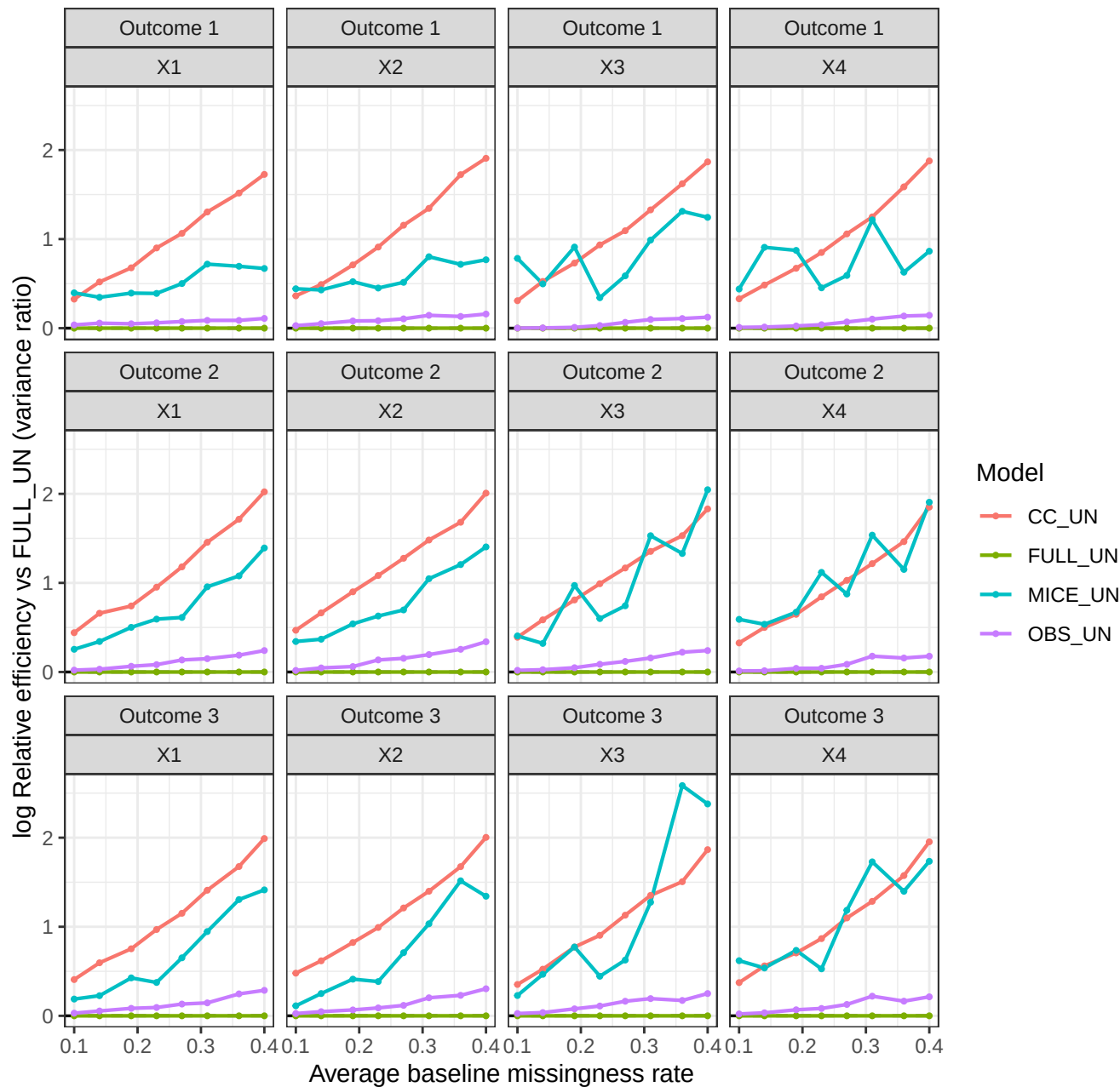
Relative efficiency of beta estimates across methods and missingness
