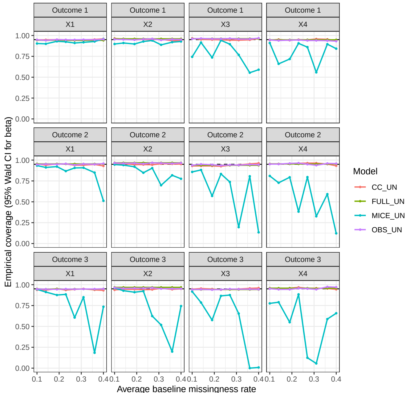
Coverage of nominal 95% CIs for beta by method
