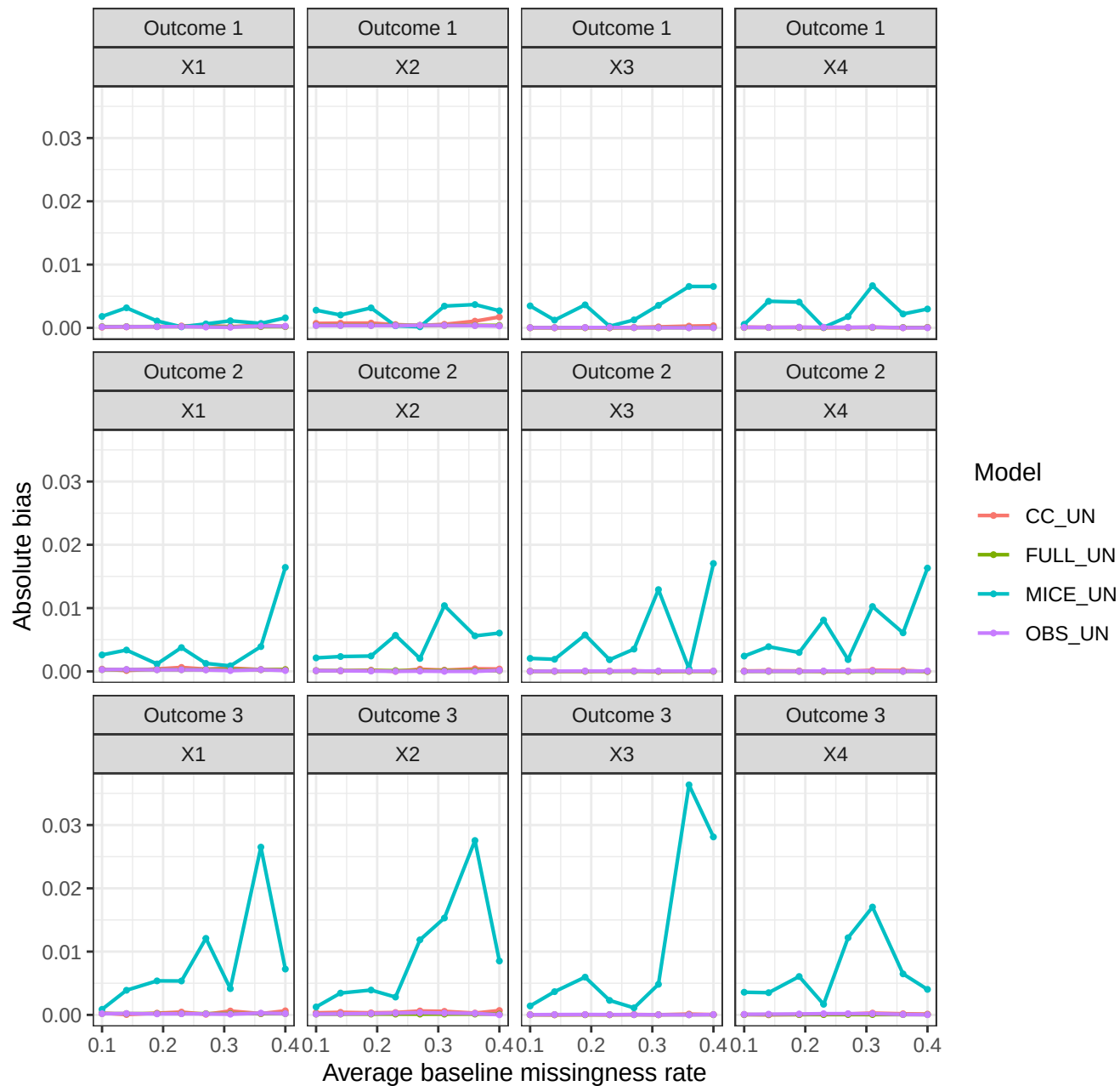
Bias of beta estimates across methods and missingness
